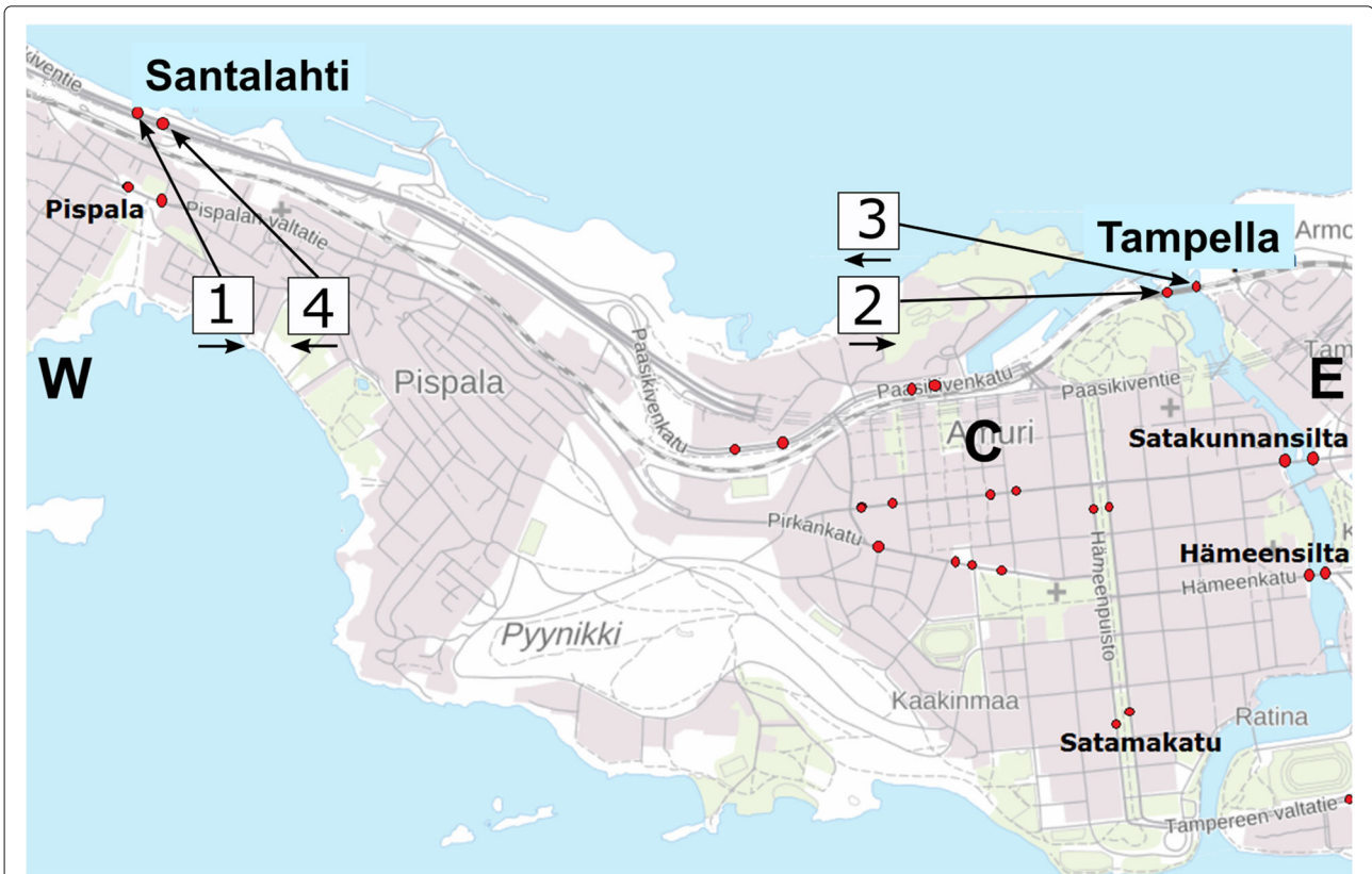
Fig. 5 Illustration of inductive loop measurement points in the city of Tampere. This research utilises locations Santalahti and Tampella and our measurement points are denoted as in Fig 1. The city centre, denoted by C, is located at southwest of Tampella
