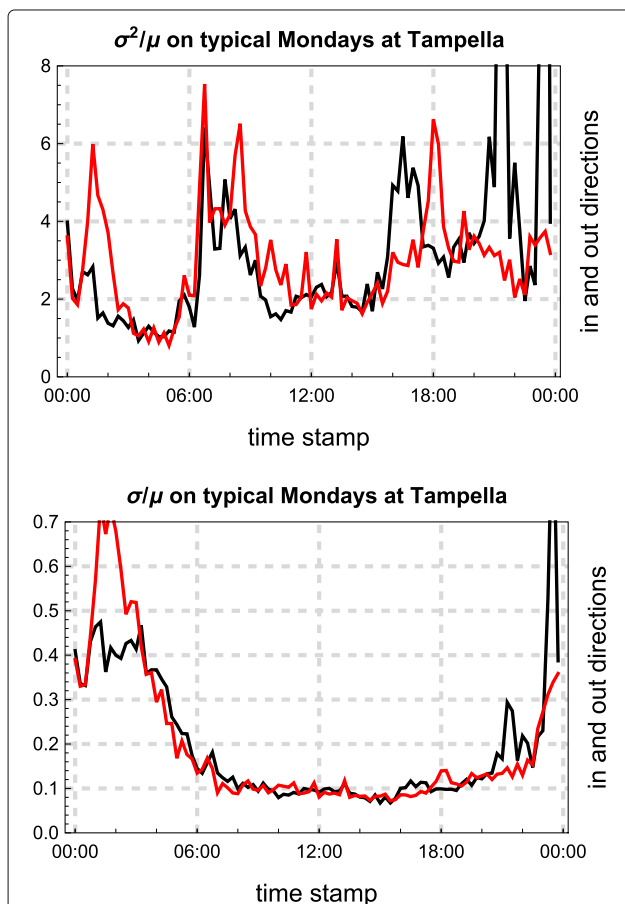
Fig. 2 The index of dispersion (IDC, \sigma^2/\mu , upper) and the coefficient of variation (CoV, \sigma/\mu , lower) of the observed vehicle counts are illustrated on normal working day Mondays at Tampella measurement point. Inbound and outbound traffic are illustrated in black and red, respectively
